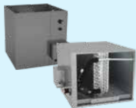
Serpentins en aluminium Daikin (CAPE/CAPEA/CHPE)
